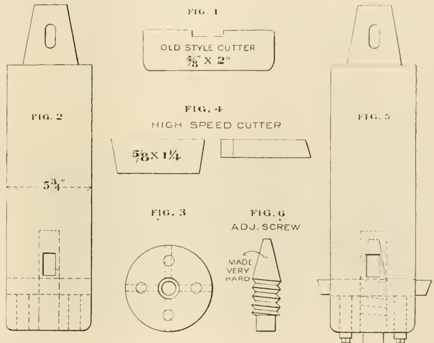
CUTTING TOOLS FOR CAR WHEELS.
